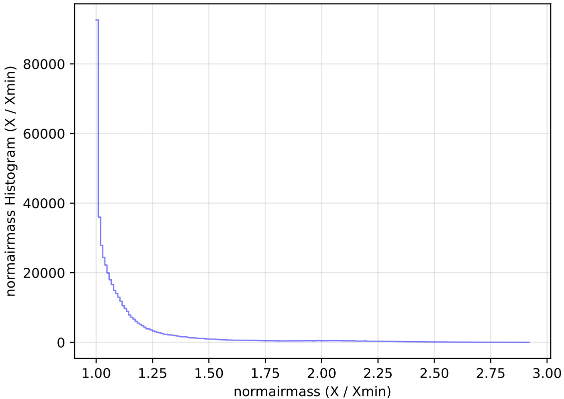
smc_lmc_v3.3_10yrs WFD i band: normairmass Histogram
