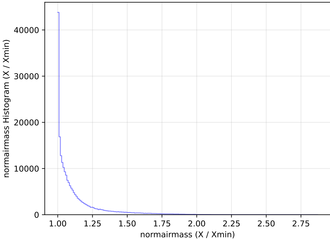
smc_lmc_v3.3_10yrs WFD g band: normairmass Histogram
