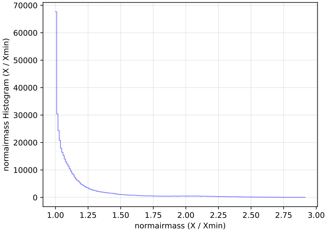
smc_lmc_v3.3_10yrs All sky z band: normairmass Histogram
