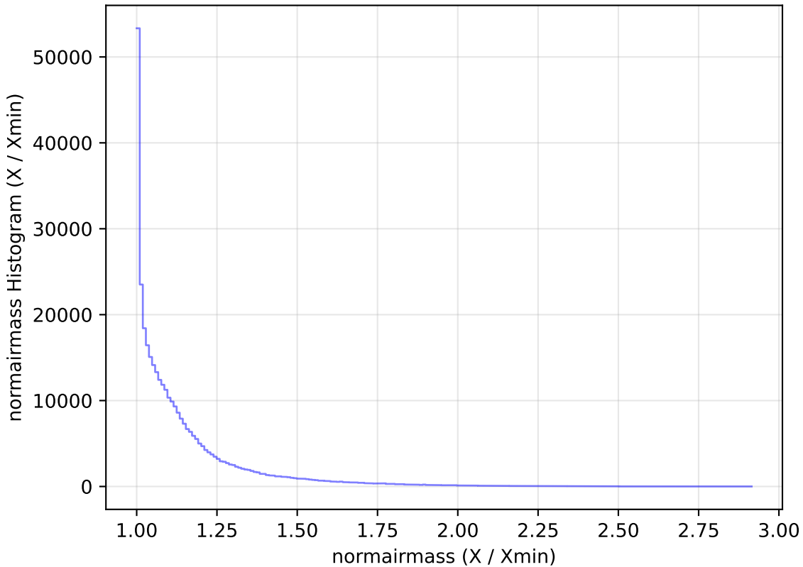
smc_lmc_v3.3_10yrs All sky y band: normairmass Histogram
