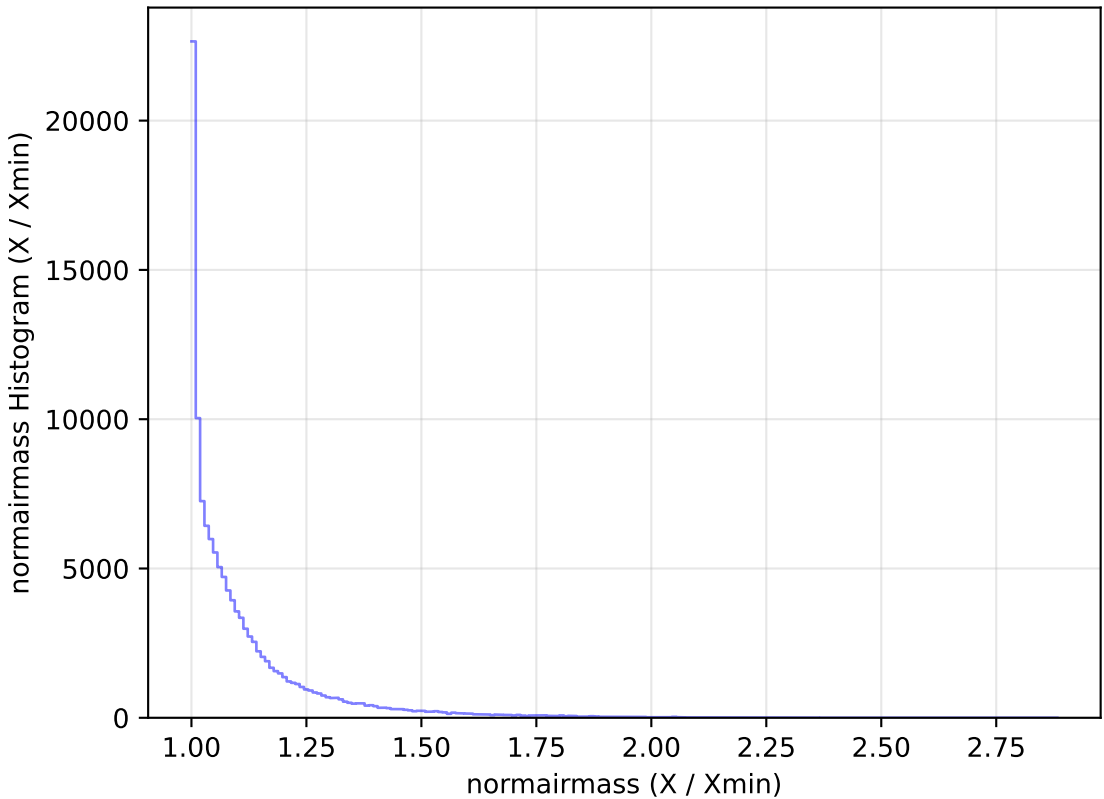
smc_lmc_v3.3_10yrs All sky u band: normairmass Histogram
