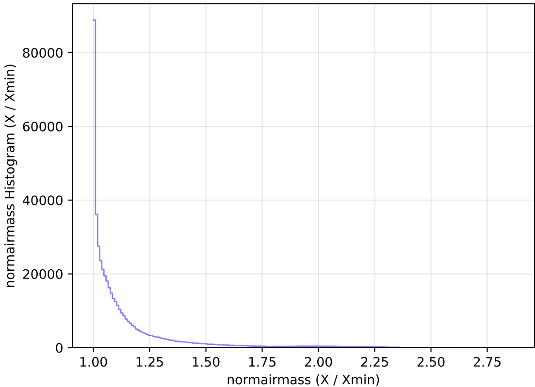
smc_lmc_v3.3_10yrs All sky r band: normairmass Histogram
