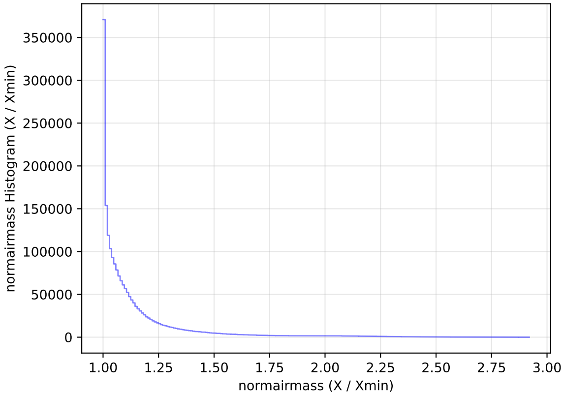
smc_lmc_v3.3_10yrs All sky all bands: normairmass Histogram
