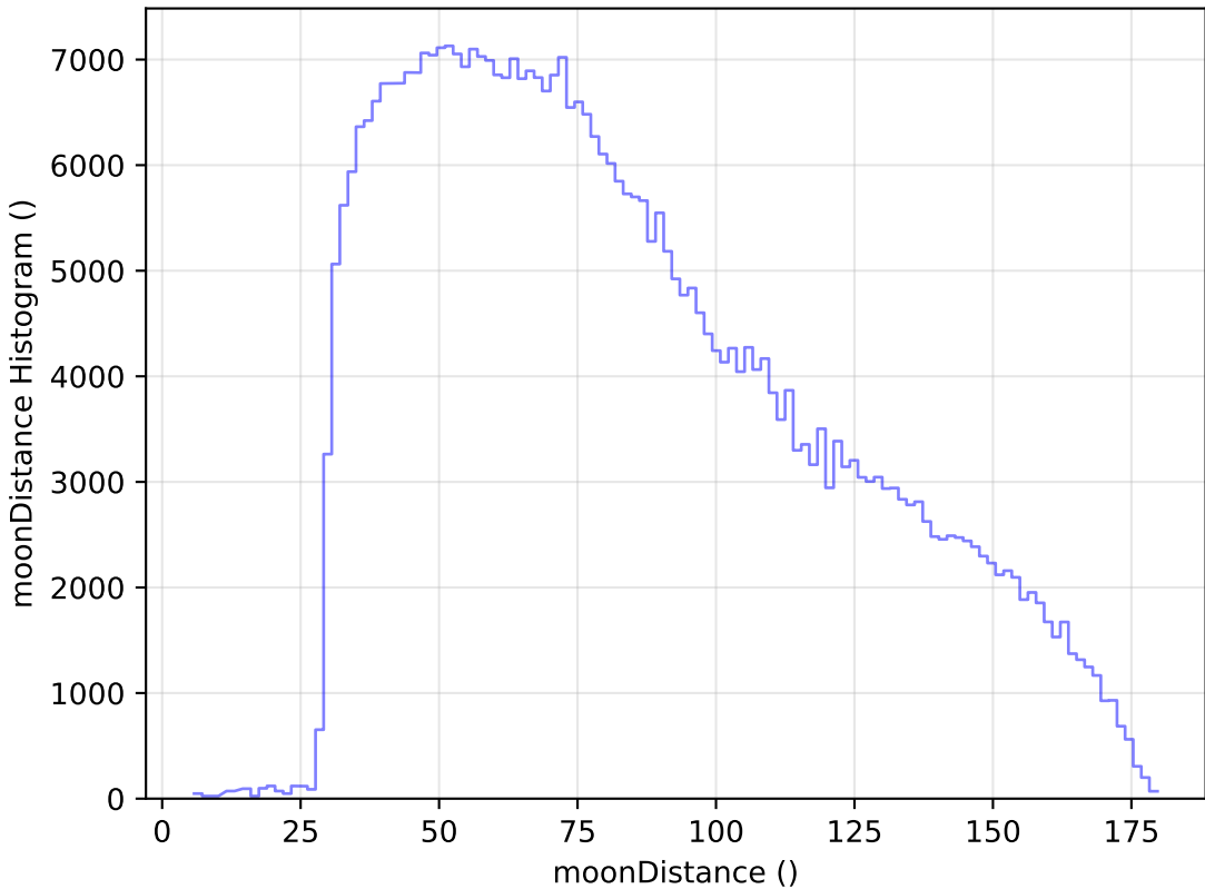
smc_lmc_v3.3_10yrs WFD z band: moonDistance Histogram
