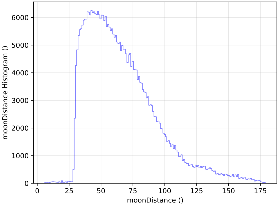
smc_lmc_v3.3_10yrs WFD y band: moonDistance Histogram
