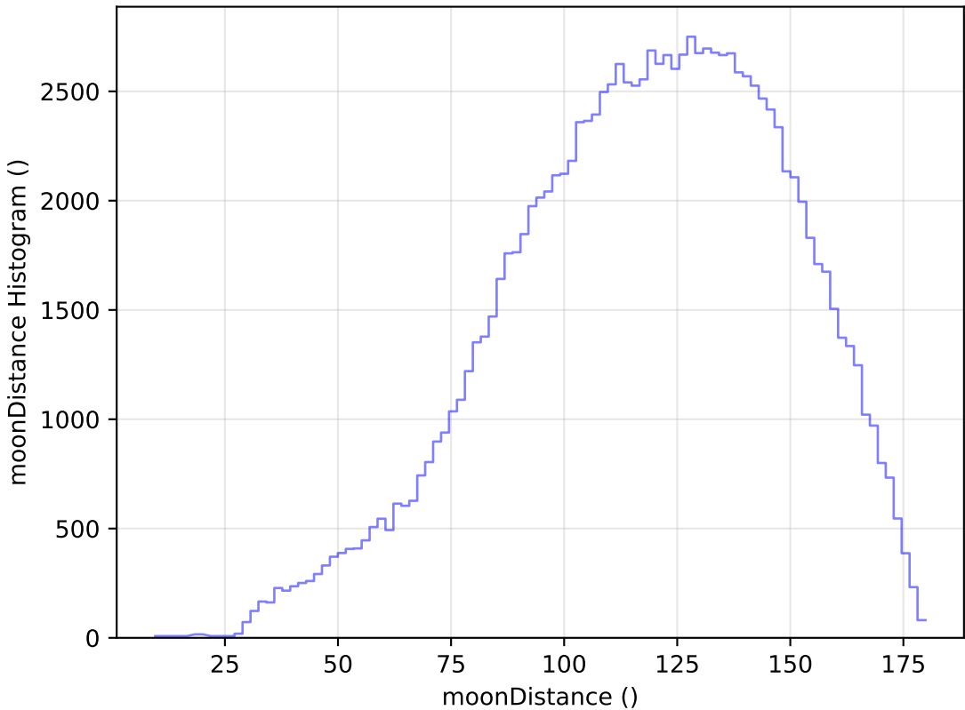
smc_lmc_v3.3_10yrs WFD u band: moonDistance Histogram
