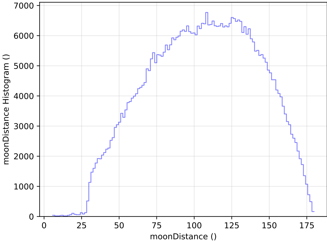
smc_lmc_v3.3_10yrs WFD r band: moonDistance Histogram
