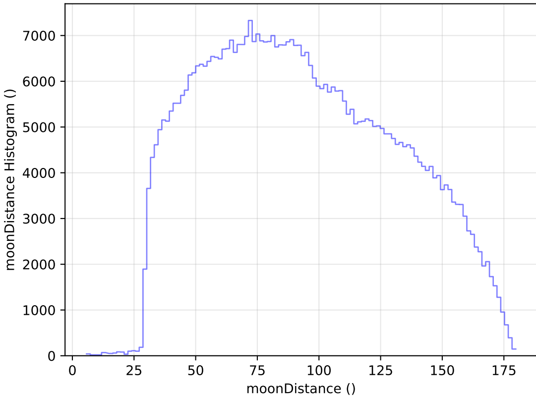
smc_lmc_v3.3_10yrs WFD i band: moonDistance Histogram
