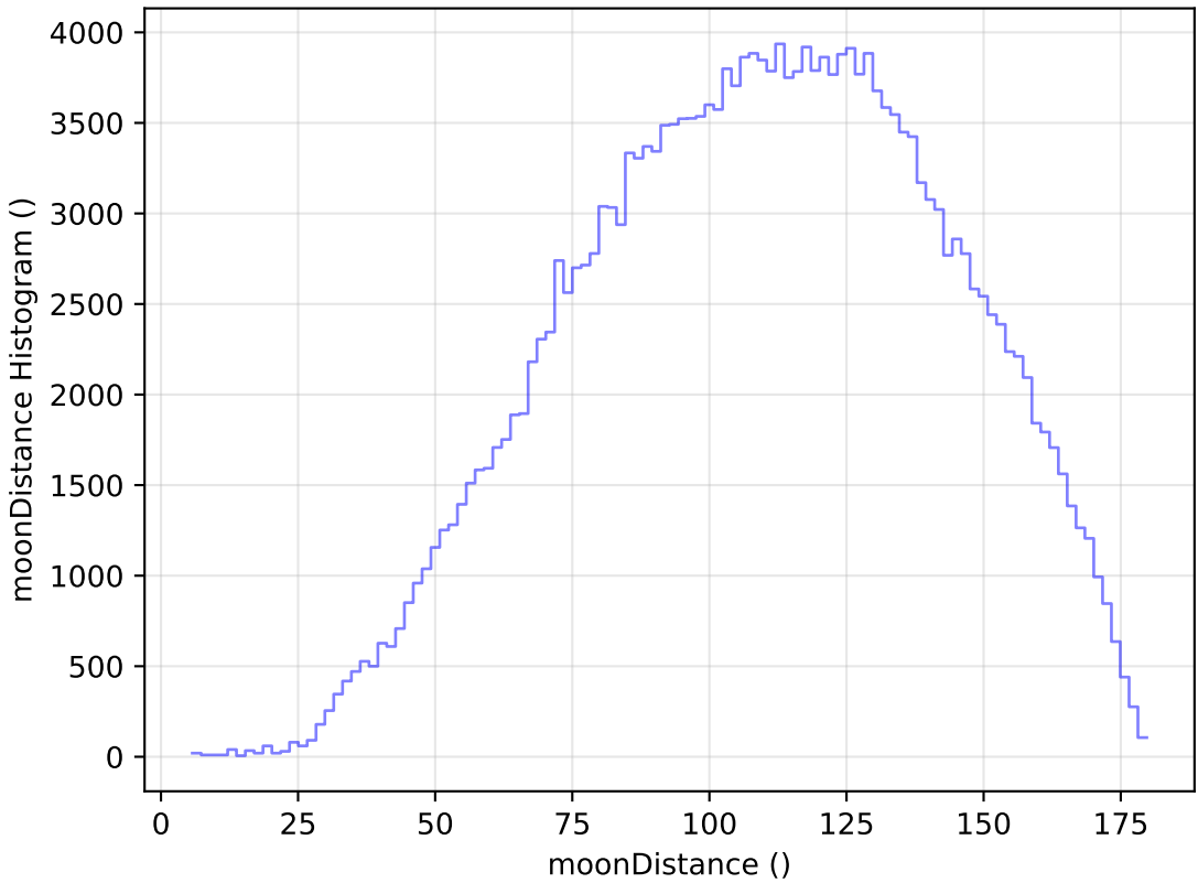
smc_lmc_v3.3_10yrs WFD g band: moonDistance Histogram
