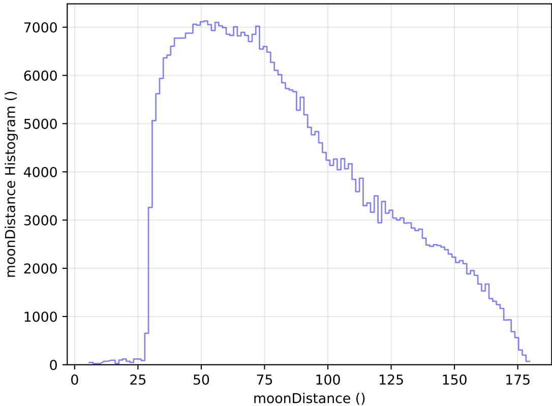
smc_lmc_v3.3_10yrs All sky z band: moonDistance Histogram
