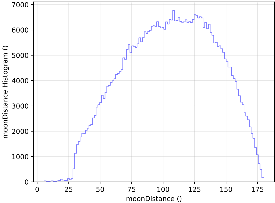
smc_lmc_v3.3_10yrs All sky r band: moonDistance Histogram
