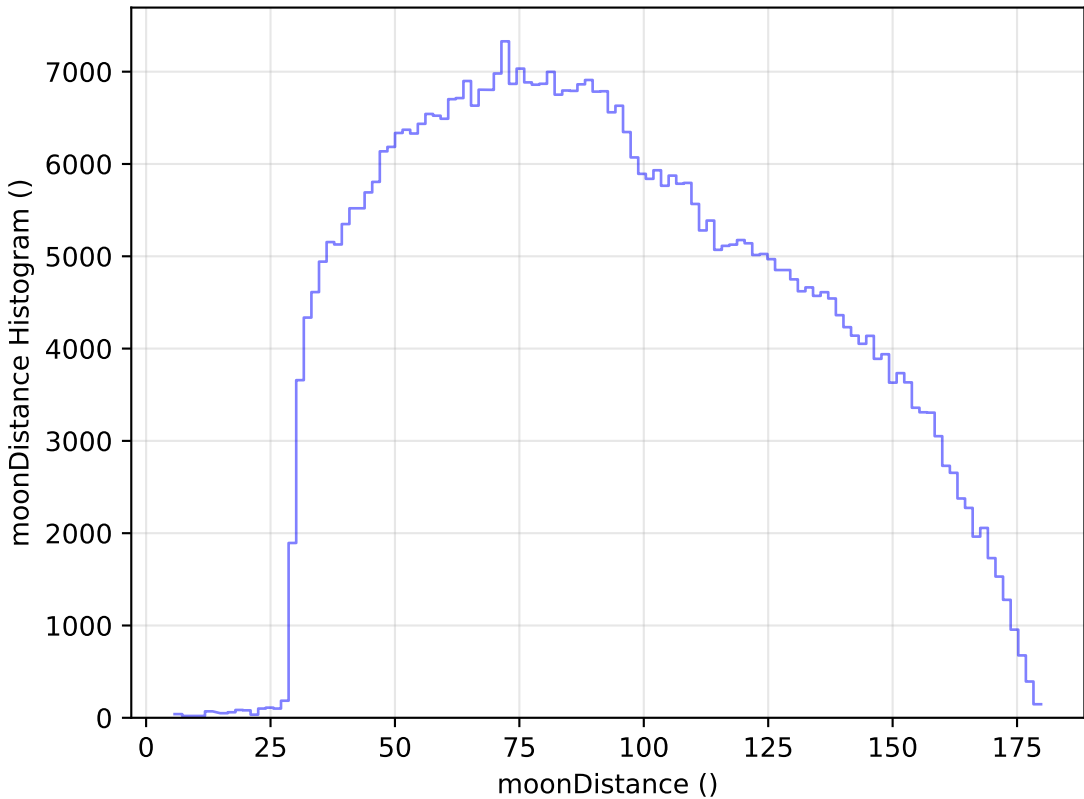
smc_lmc_v3.3_10yrs All sky i band: moonDistance Histogram
