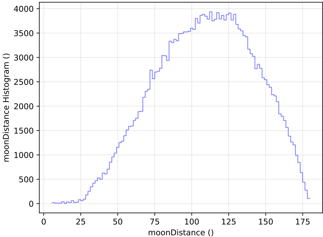
smc_lmc_v3.3_10yrs All sky g band: moonDistance Histogram
