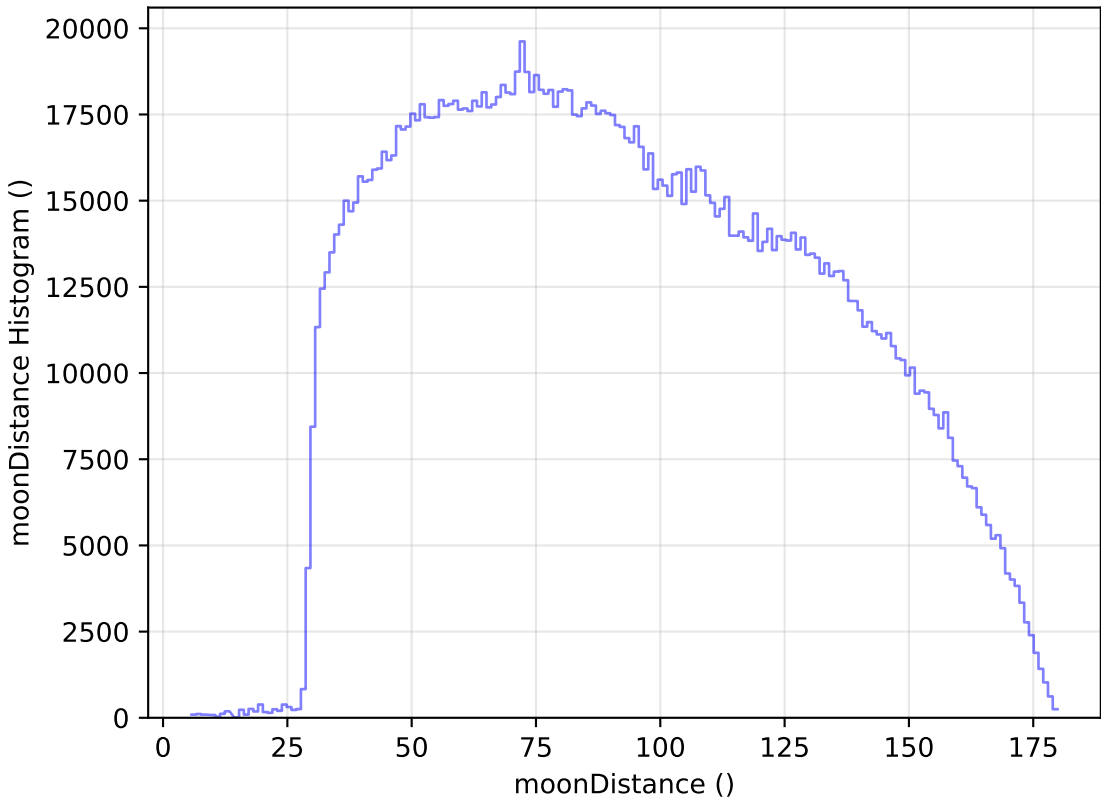
smc_lmc_v3.3_10yrs All sky all bands: moonDistance Histogram
