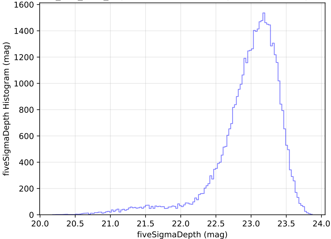
smc_lmc_v3.3_10yrs Yr 1 z band: fiveSigmaDepth Histogram
