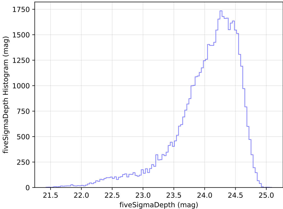
smc_lmc_v3.3_10yrs Yr 1 r band: fiveSigmaDepth Histogram
