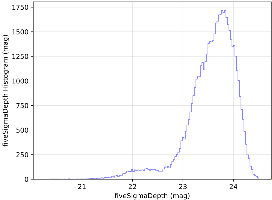
smc_lmc_v3.3_10yrs Yr 1 i band: fiveSigmaDepth Histogram
