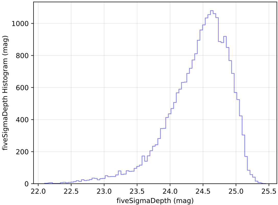
smc_lmc_v3.3_10yrs Yr 1 g band: fiveSigmaDepth Histogram
