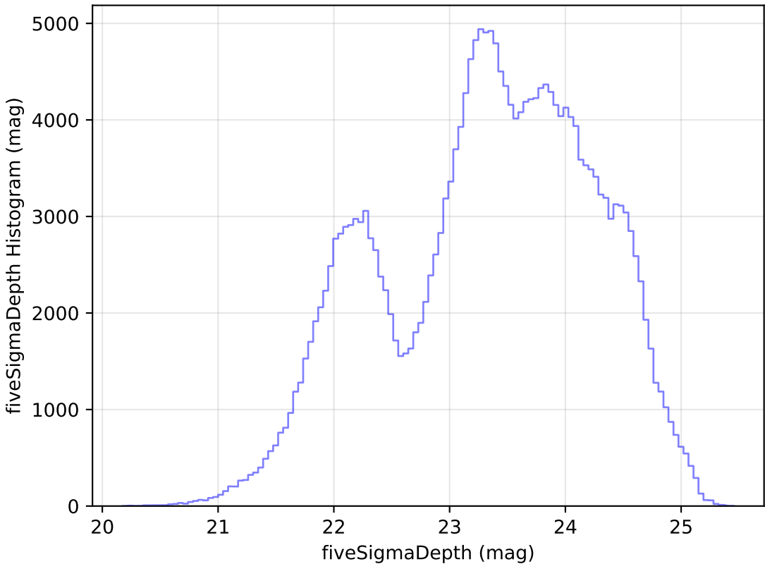
smc_lmc_v3.3_10yrs Yr 1 all bands: fiveSigmaDepth Histogram
