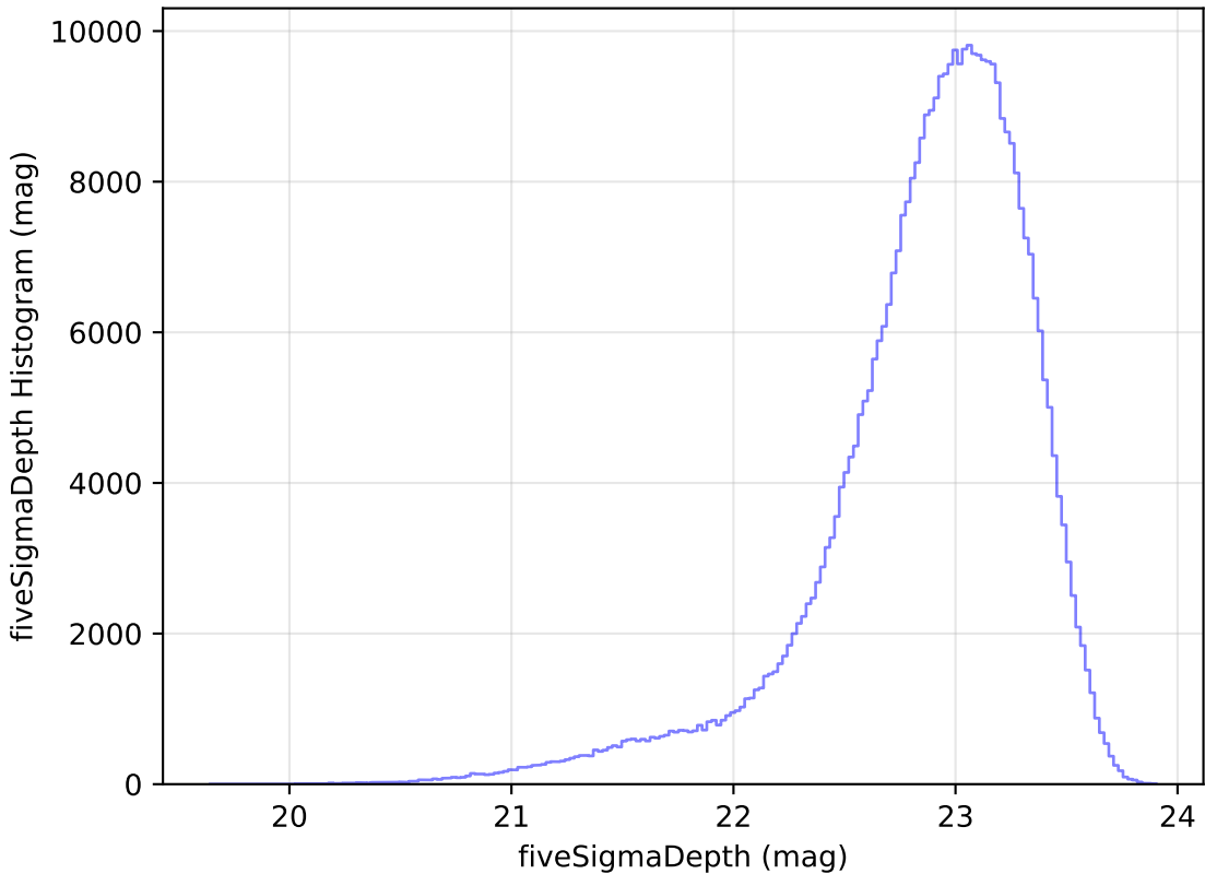
smc_lmc_v3.3_10yrs WFD z band: fiveSigmaDepth Histogram
