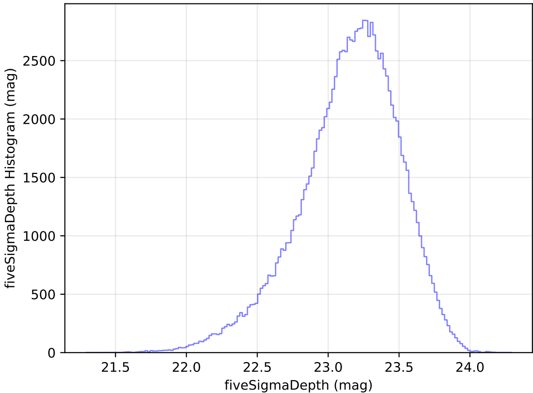
smc_lmc_v3.3_10yrs WFD u band: fiveSigmaDepth Histogram
