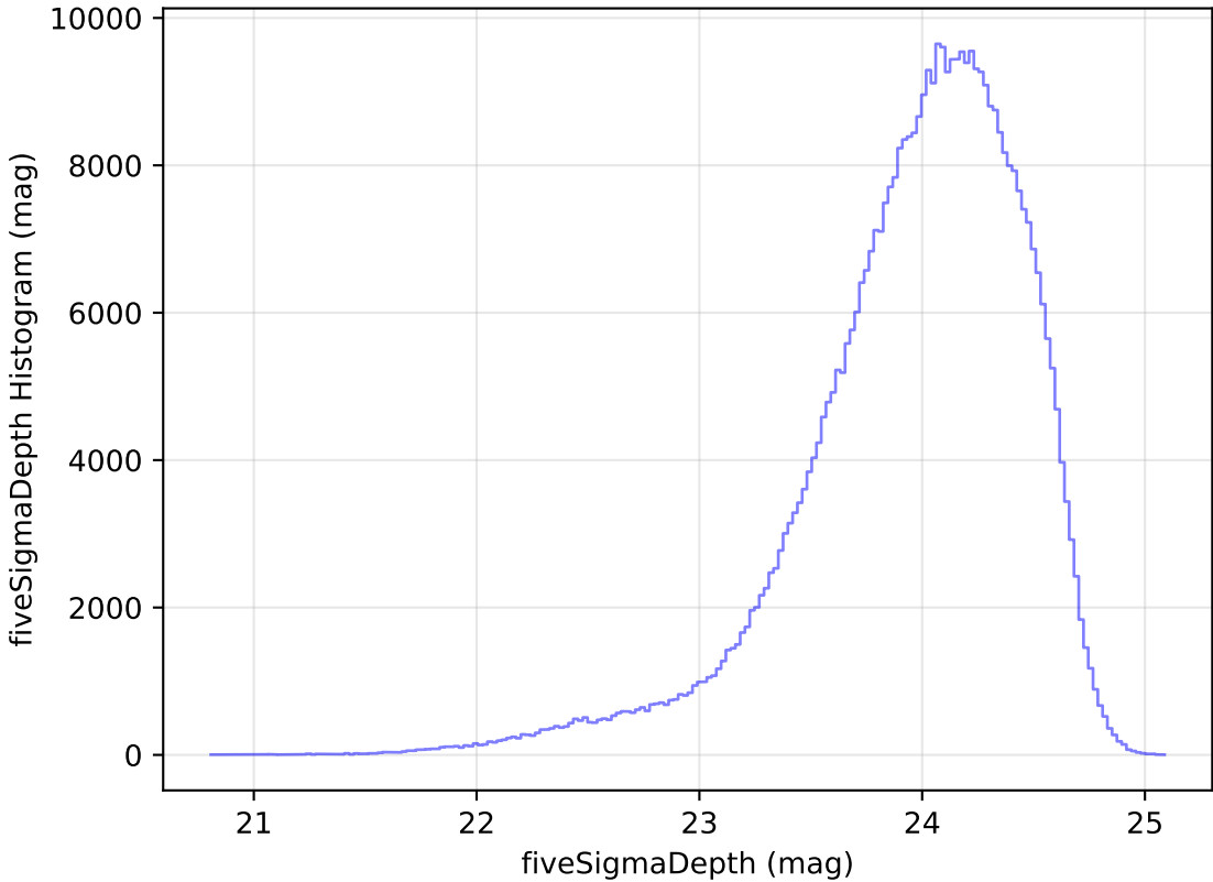
smc_lmc_v3.3_10yrs WFD r band: fiveSigmaDepth Histogram
