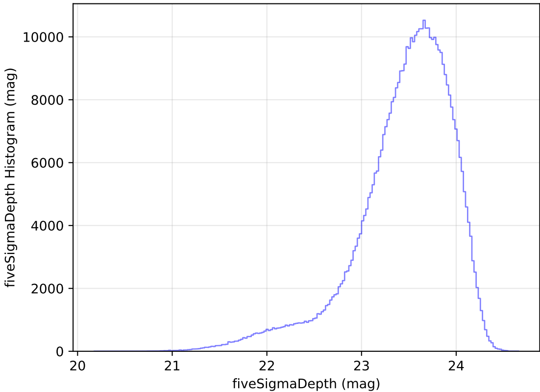
smc_lmc_v3.3_10yrs WFD i band: fiveSigmaDepth Histogram
