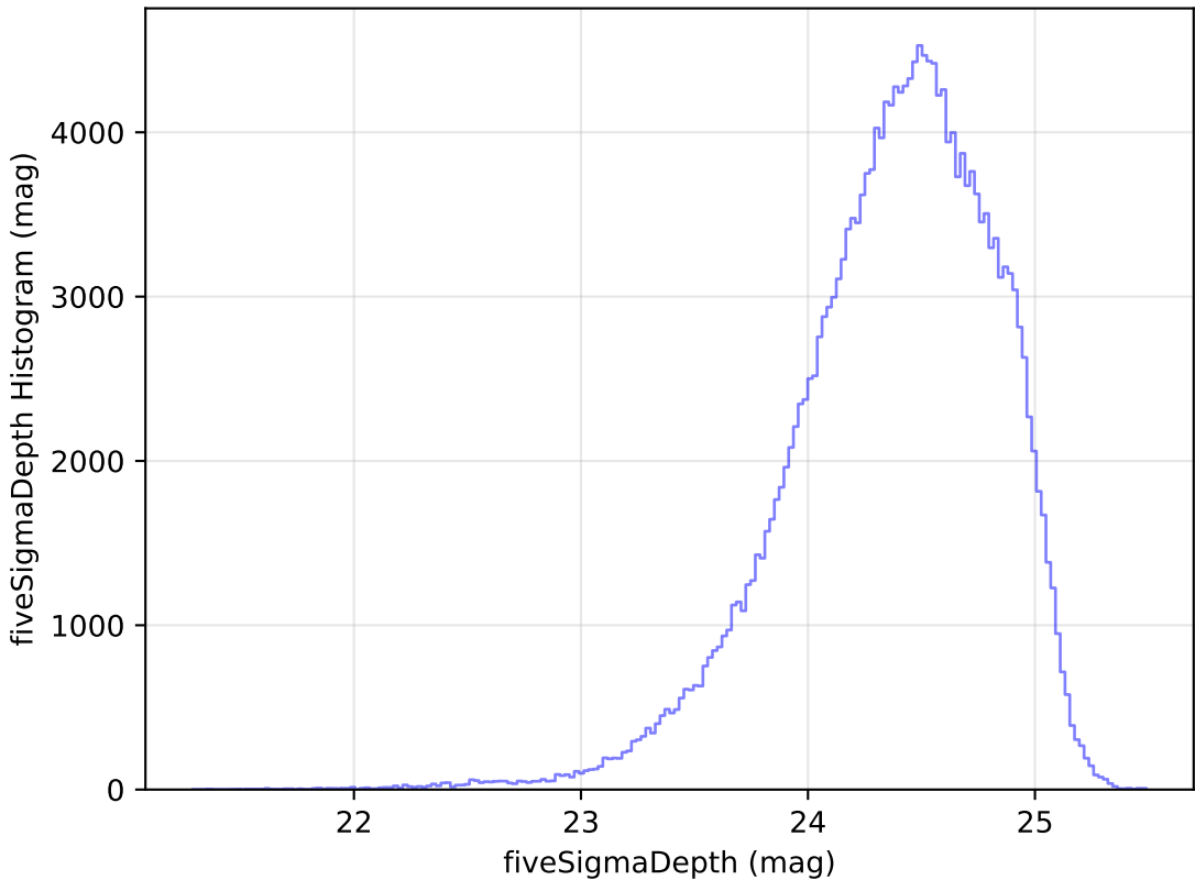
smc_lmc_v3.3_10yrs WFD g band: fiveSigmaDepth Histogram
