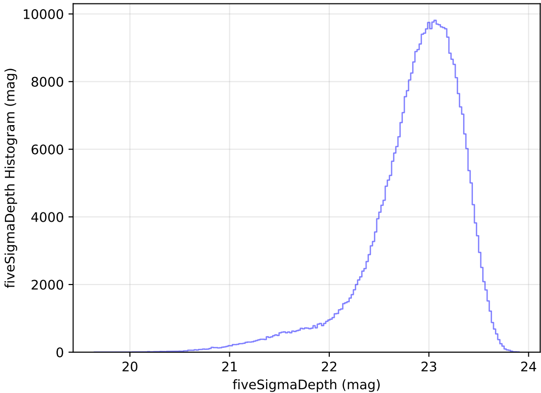
smc_lmc_v3.3_10yrs All sky z band: fiveSigmaDepth Histogram
