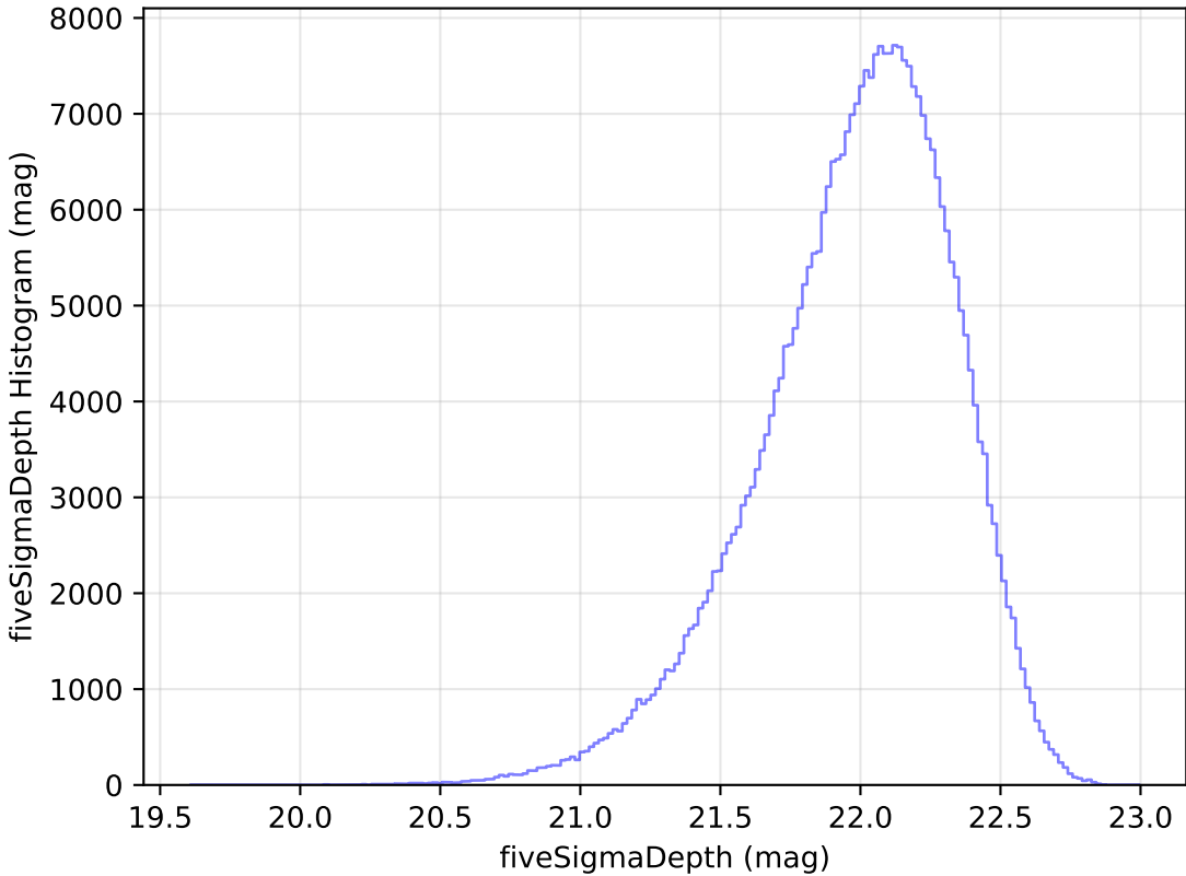
smc_lmc_v3.3_10yrs All sky y band: fiveSigmaDepth Histogram
