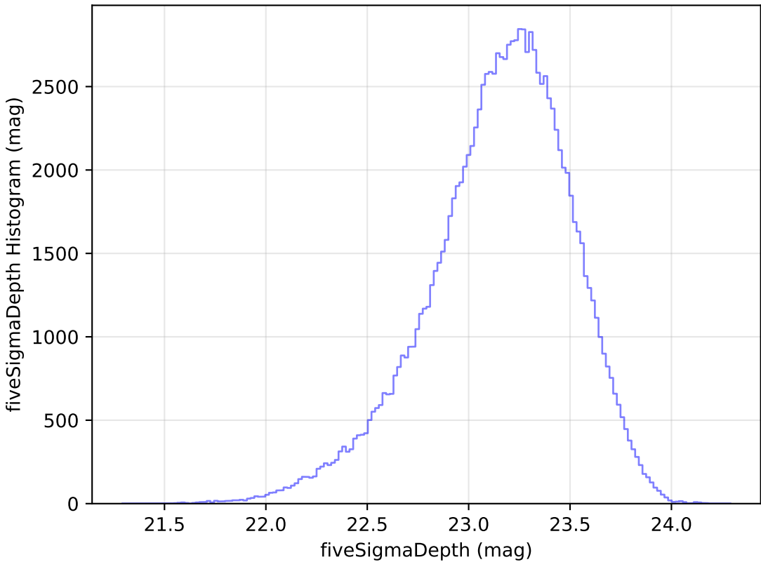
smc_lmc_v3.3_10yrs All sky u band: fiveSigmaDepth Histogram
