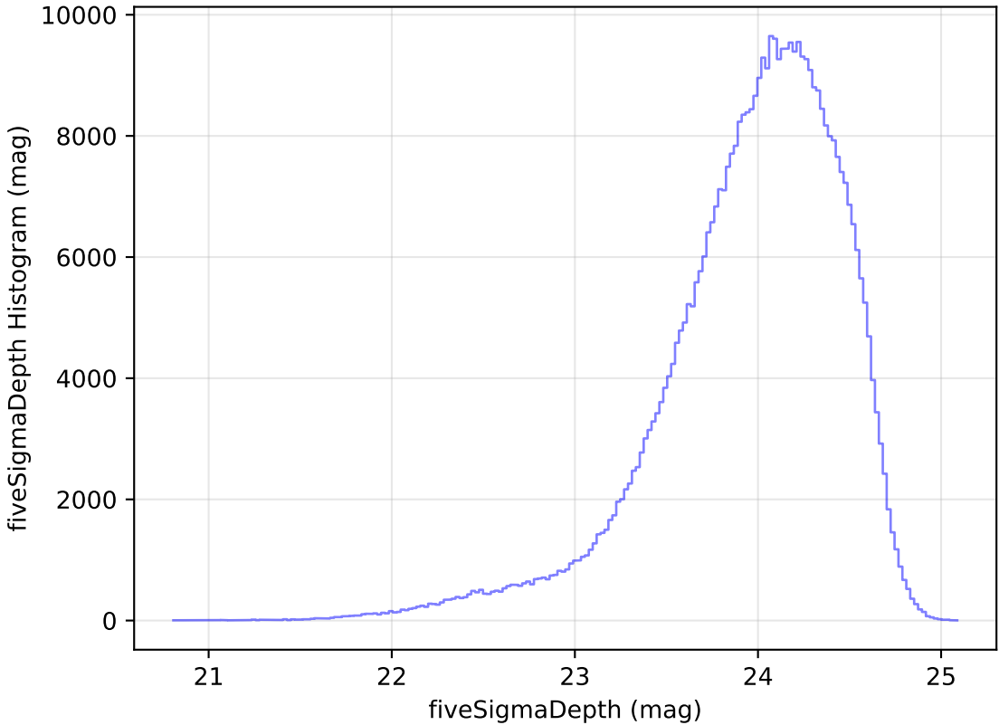
smc_lmc_v3.3_10yrs All sky r band: fiveSigmaDepth Histogram
