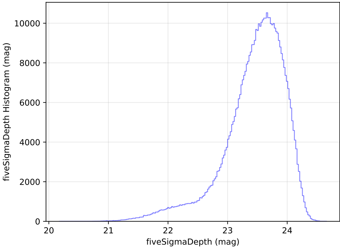
smc_lmc_v3.3_10yrs All sky i band: fiveSigmaDepth Histogram
