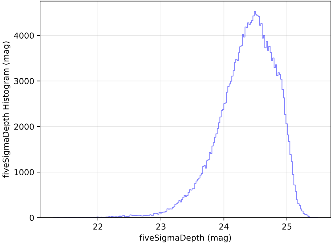
smc_lmc_v3.3_10yrs All sky g band: fiveSigmaDepth Histogram
