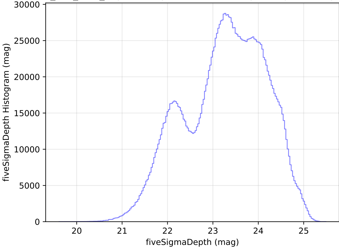
smc_lmc_v3.3_10yrs All sky all bands: fiveSigmaDepth Histogram
