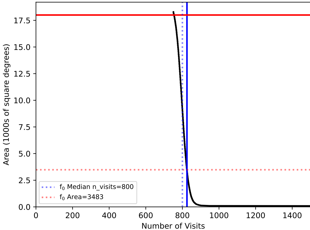
smc_lmc_v3.3_10yrs WFD: f0
