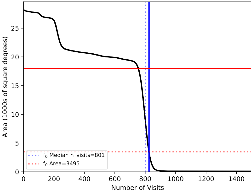
smc_lmc_v3.3_10yrs All sky: f0
