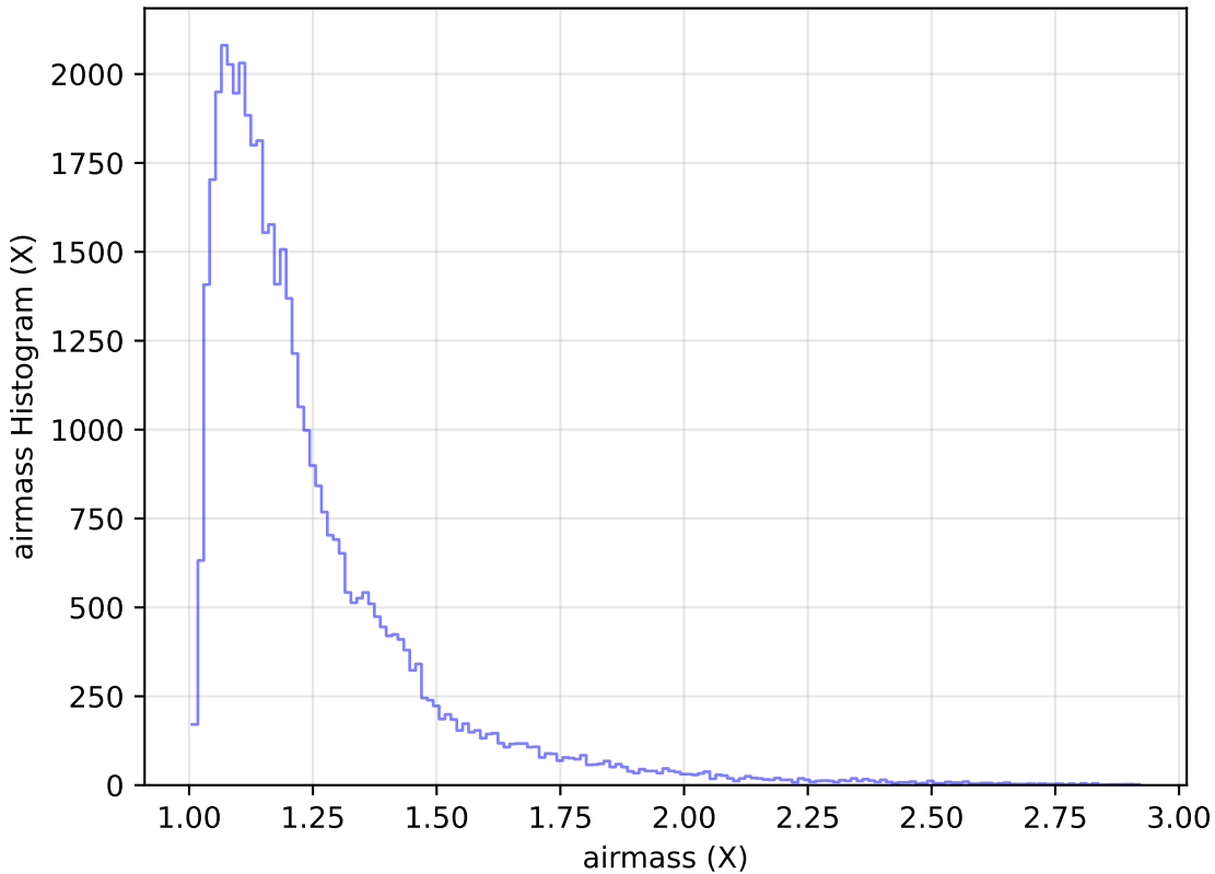
smc_lmc_v3.3_10yrs Yr 1 y band: airmass Histogram
