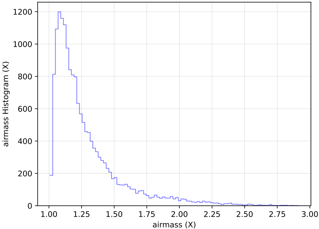
smc_lmc_v3.3_10yrs Yr 1 u band: airmass Histogram
