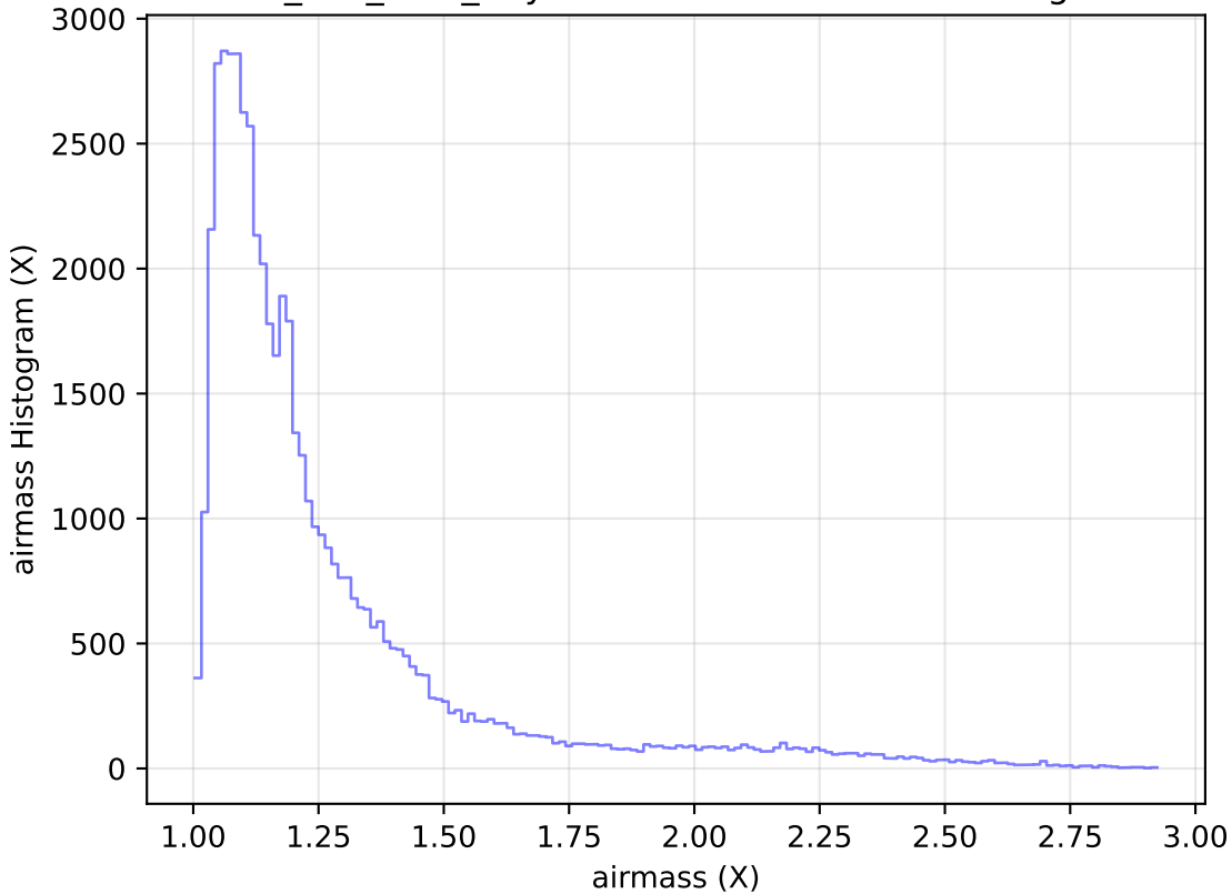
smc_lmc_v3.3_10yrs Yr 1 i band: airmass Histogram
