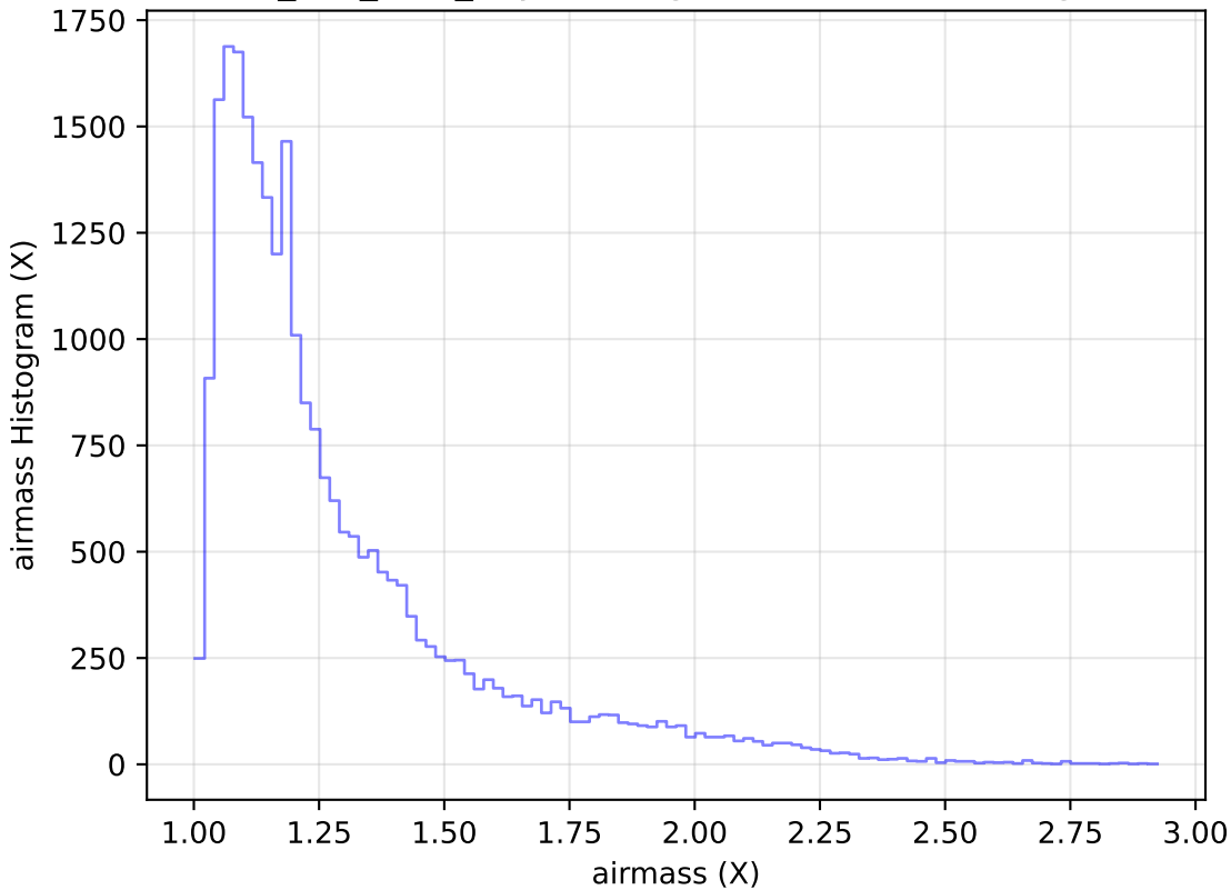
smc_lmc_v3.3_10yrs Yr 1 g band: airmass Histogram
