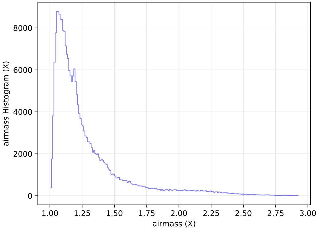
smc_lmc_v3.3_10yrs Yr 1 all bands: airmass Histogram
