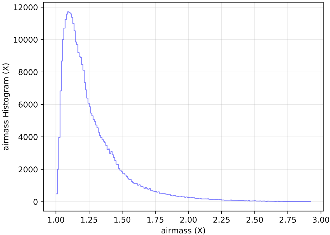
smc_lmc_v3.3_10yrs WFD y band: airmass Histogram
