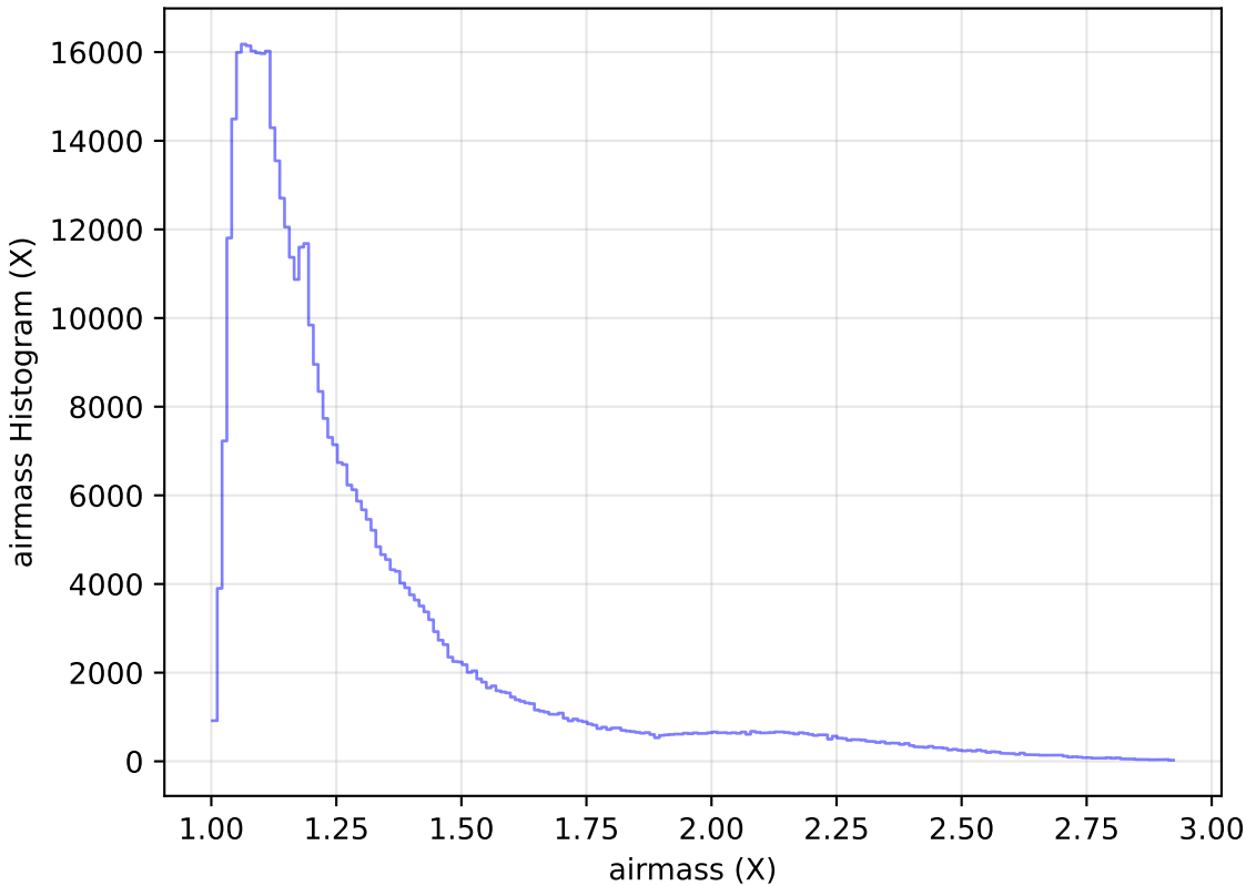
smc_lmc_v3.3_10yrs WFD i band: airmass Histogram
