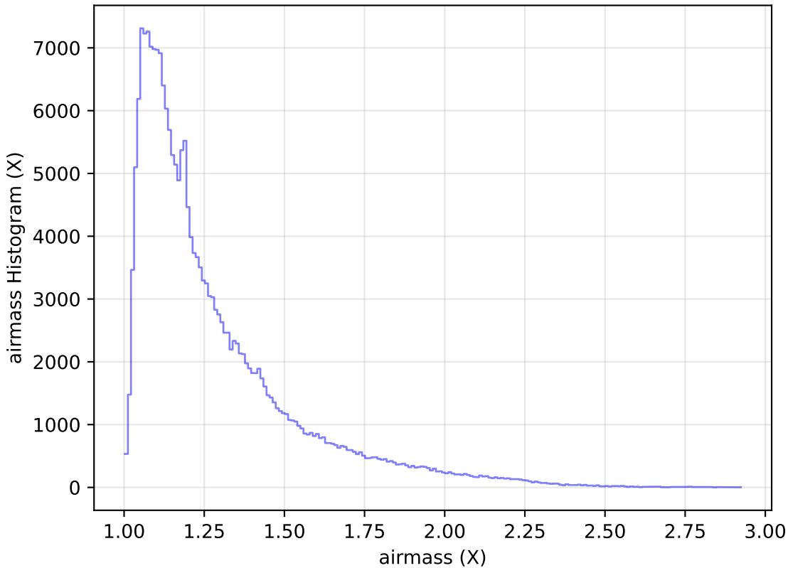
smc_Imc_v3.3_10yrs WFD g band: airmass Histogram
