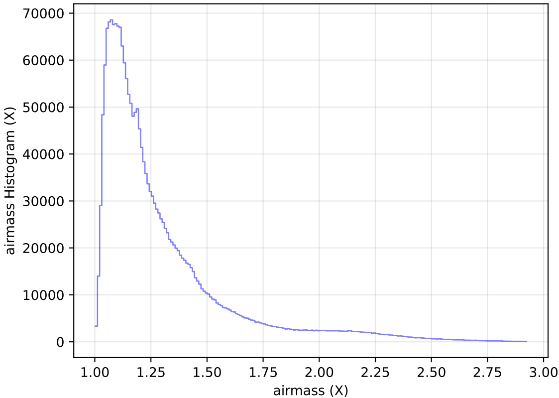
smc_lmc_v3.3_10yrs WFD all bands: airmass Histogram
