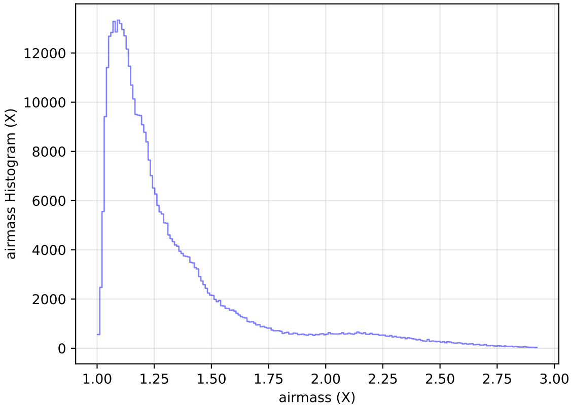
smc_lmc_v3.3_10yrs All sky z band: airmass Histogram
