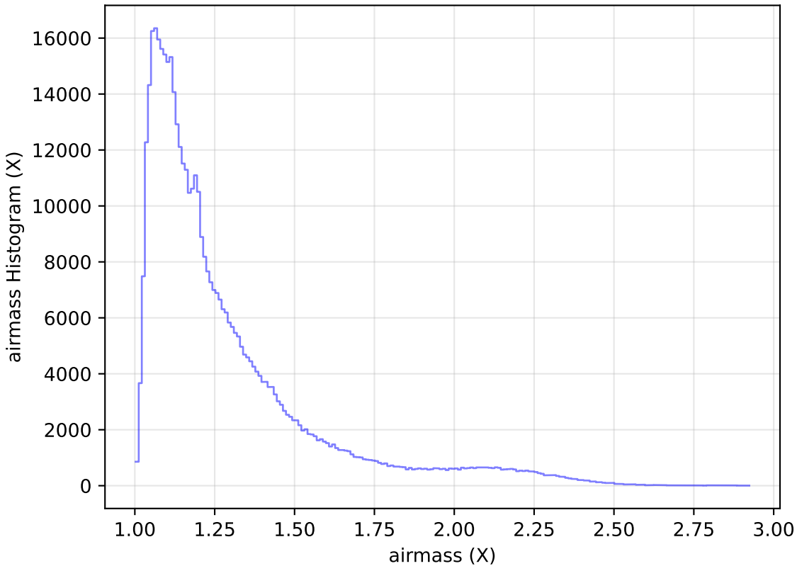
smc_lmc_v3.3_10yrs All sky r band: airmass Histogram
