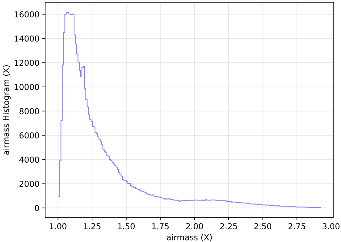
smc_lmc_v3.3_10yrs All sky i band: airmass Histogram
