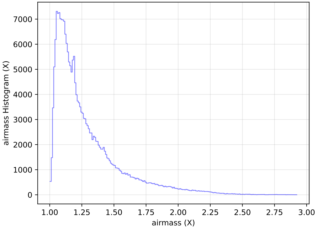
smc_lmc_v3.3_10yrs All sky g band: airmass Histogram
